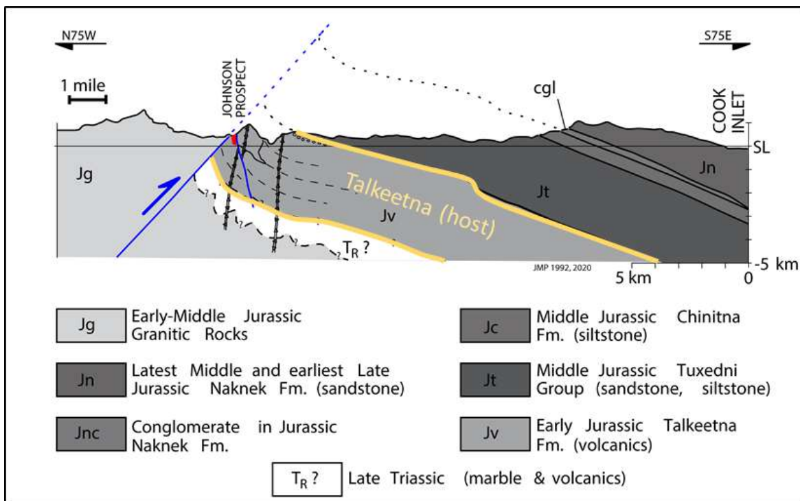
Figure 7.2 Schematic cross-section of the regional geology of the Johnson Tract (Modified from Proffett, 2021)
