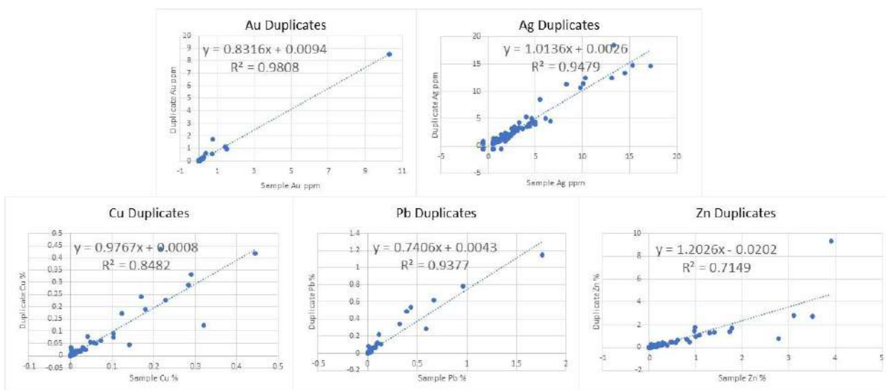
Figure 11.7 1:1 plots of duplicate assay pairs. Linear regression equations and R^2 values are shown on the plots.
