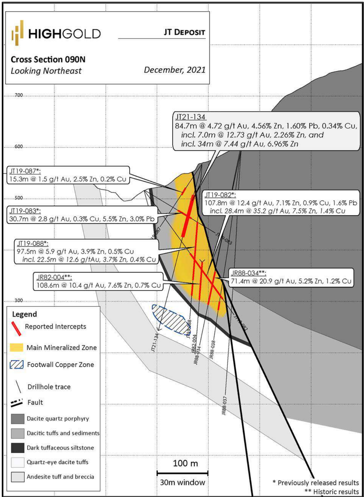
Figure 7.6 JT Project – Cross-Section of the JT Deposit Significant Drill Hole Intersections
