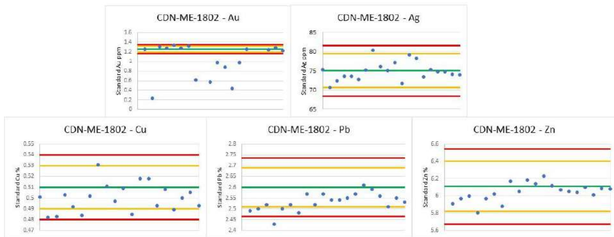
Figure 11.5 Control charts for low-grade polymetallic standard ME-1802. Mean value is plotted as green lines for each element, second standard deviations are yellow, third standard deviations are red.
