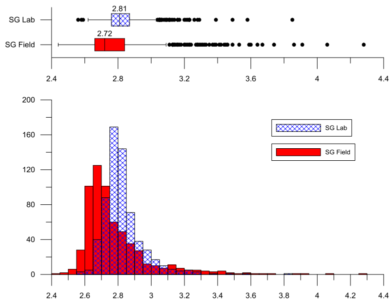
Figure 11.1 Histogram and Box and whisker plots showing all Lab and Field SG data.
