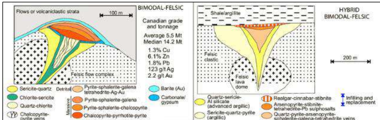
Figure 8.3 VMS Deposit Model from Gallery et al., 2007.
