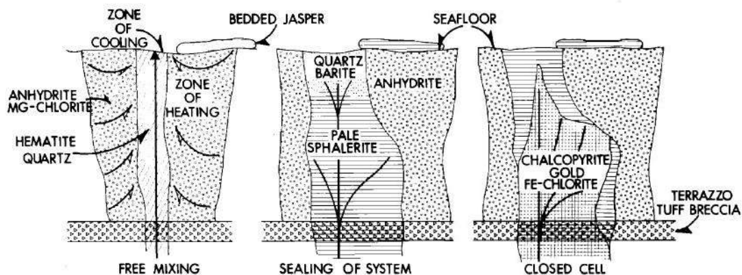
Figure 8.1 Genetic model of the hydrothermal system at the Johnson Tract deposit from Steefel (1987)
