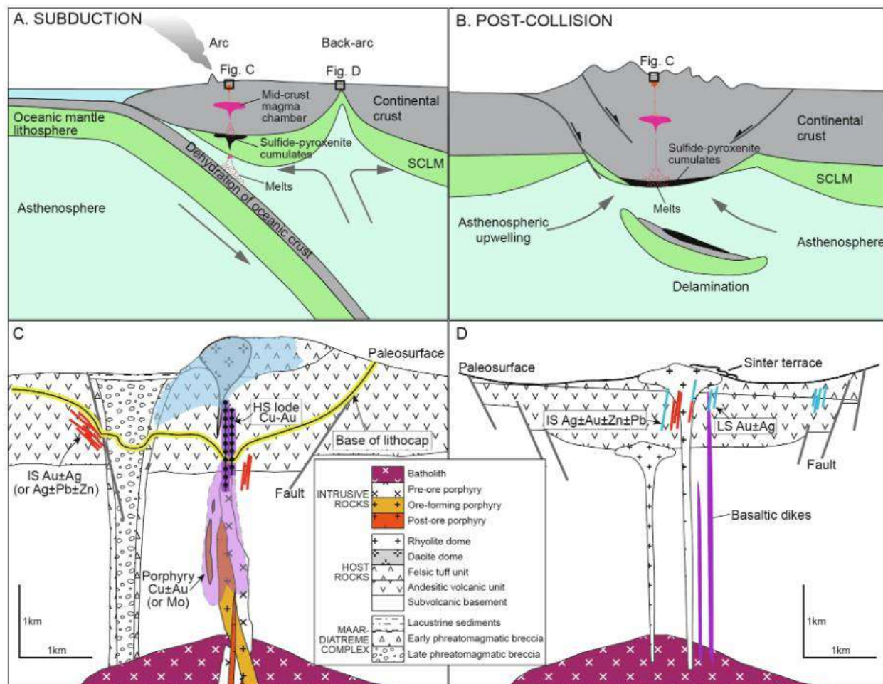
Figure 8.4 Schematic diagram showing the setting of intermediate sulphidation subtypes from Wang et al., 2019
