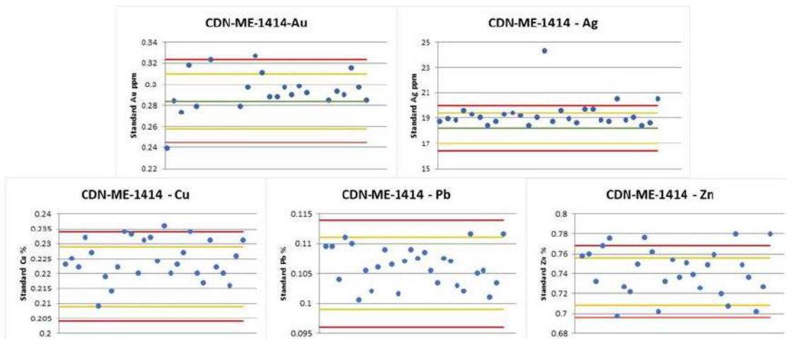
Figure 11.4 Control charts for low-grade polymetallic standard ME-1414. Mean value is plotted as green lines for each element, second standard deviations are yellow, third standard deviations are red.
