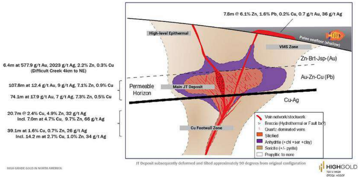
Figure 8.2 JT Deposit Model – Epithermal/VMS Hybrid from Highgold (2021)
