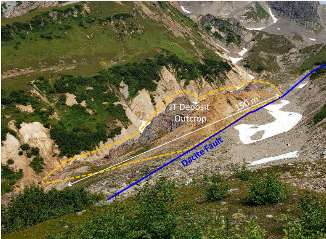
Plate 7.3 Photo of the JT Deposit surface outcrop looking northwest
