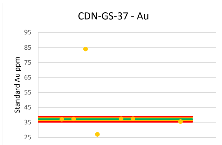
Figure 11.2 Control charts for high-grade gold standard CDN-GS-37. Mean value is potted as green lines, second standard deviations are yellow, third standard deviations are red
