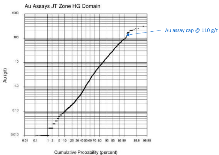
Figure 14.3 Example Histogram & Probability Plot: JT HG Domain – Au Assays
