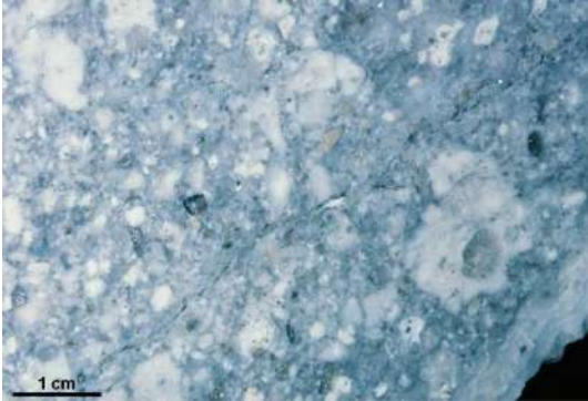
B - Dacite quartz-eye lapilli tuff (DLT)
