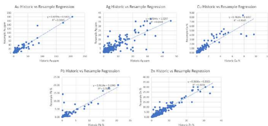
Figure 12.1 2018 Resampling Program – One-to-One Plots of Historic vs. Resample Assay Pairs
