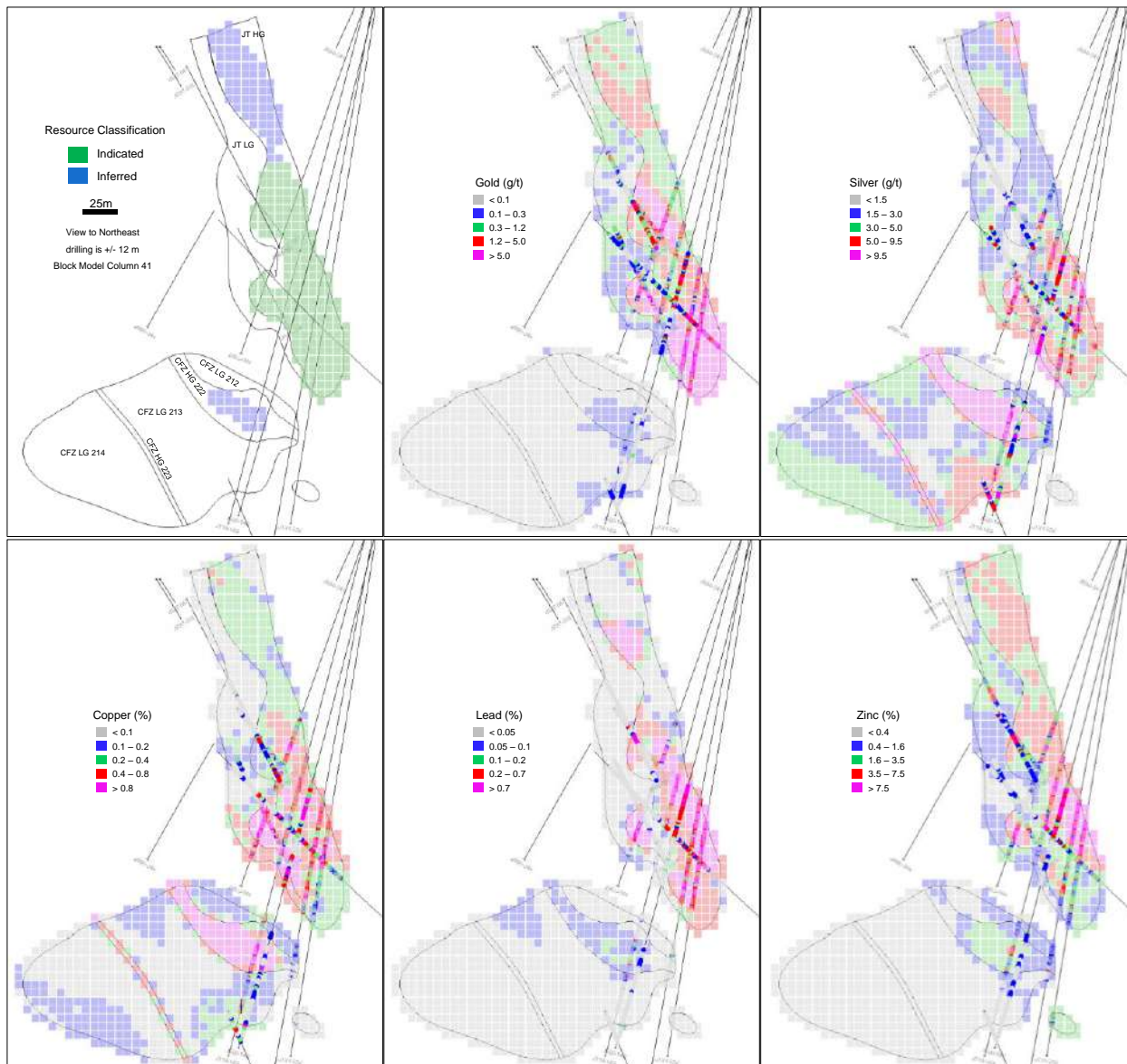
Figure 14.4 Example Section - Model Column 41: Resource Class, Block Estimate and Composite Grades
