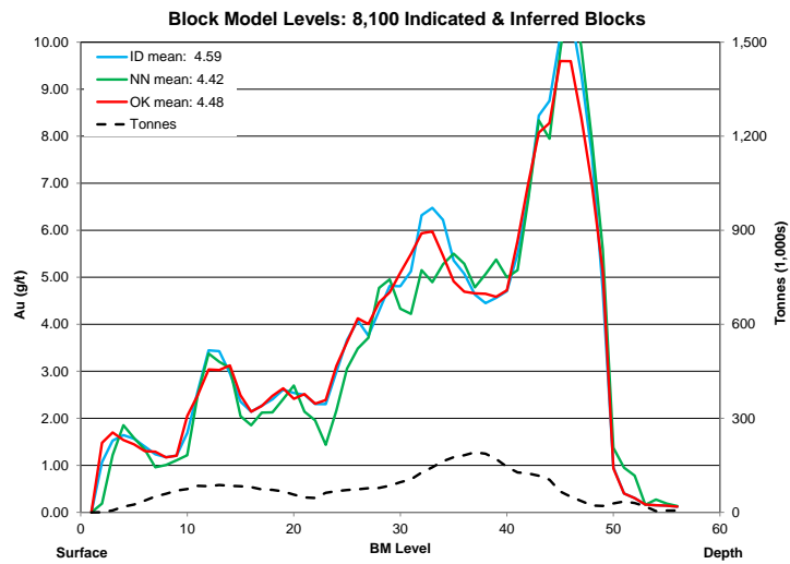
Figure 14.5 Swath Plots Comparing OK, ID and NN Models in Johnson Domain
