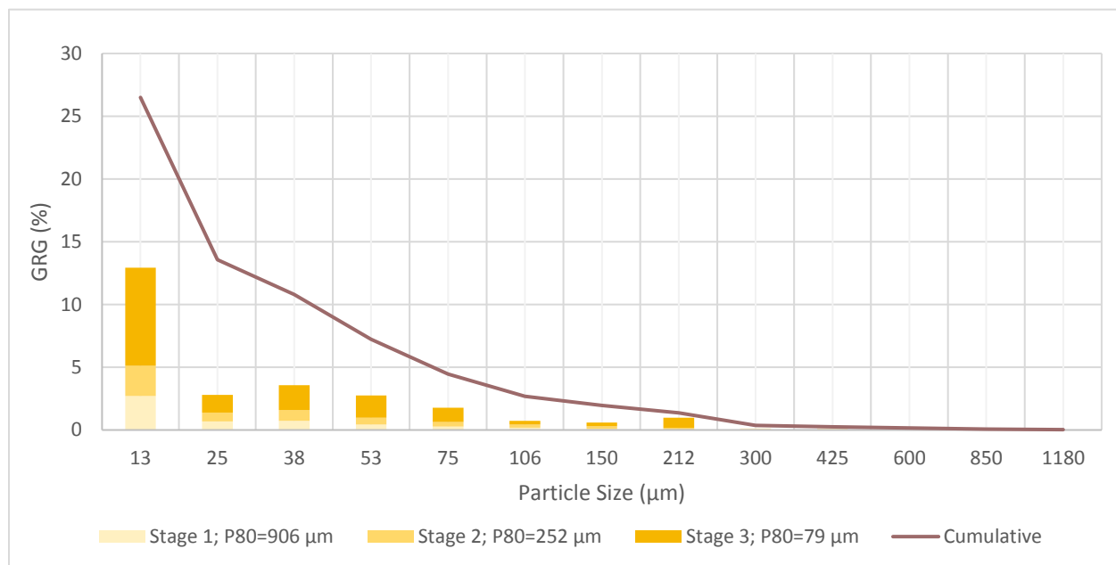
Figure 13.2: Johnson Tract Gravity Recoverable Gold by Size Fraction
