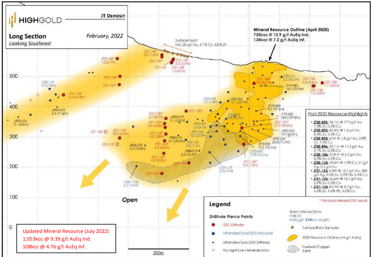
Figure 10.3 JT Deposit – Longitudinal Section with 2021 DDH Intersections
