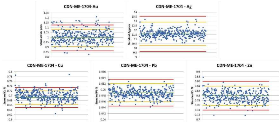
Figure 11.3 Control charts for low-grade polymetallic standard ME-1704. Mean value is plotted as green lines for each element, second standard deviations are yellow, third standard deviations are red.
