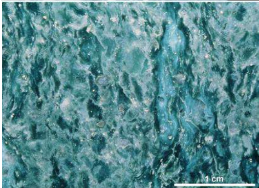
C - Dacite pumice lapilli tuff (DLT), host to mineralization
