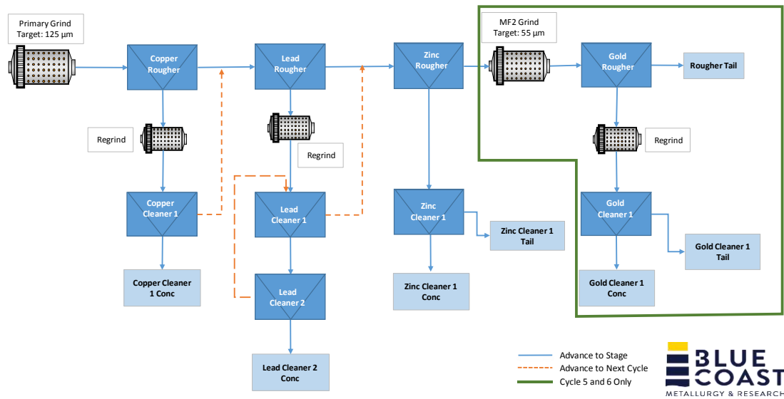
Figure 13.3: LCT-1 Flowsheet
